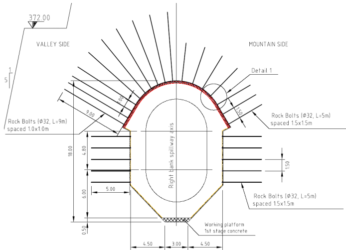
Figure 8. Rock support of the overflow spillway on the right bank.
